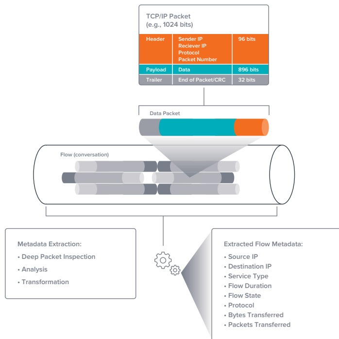
Figure 1: Metadata extraction
